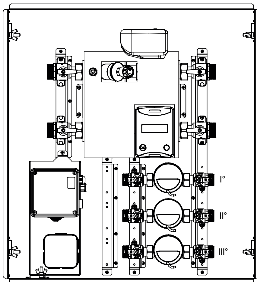
Figure 8A: Domestic water meters
