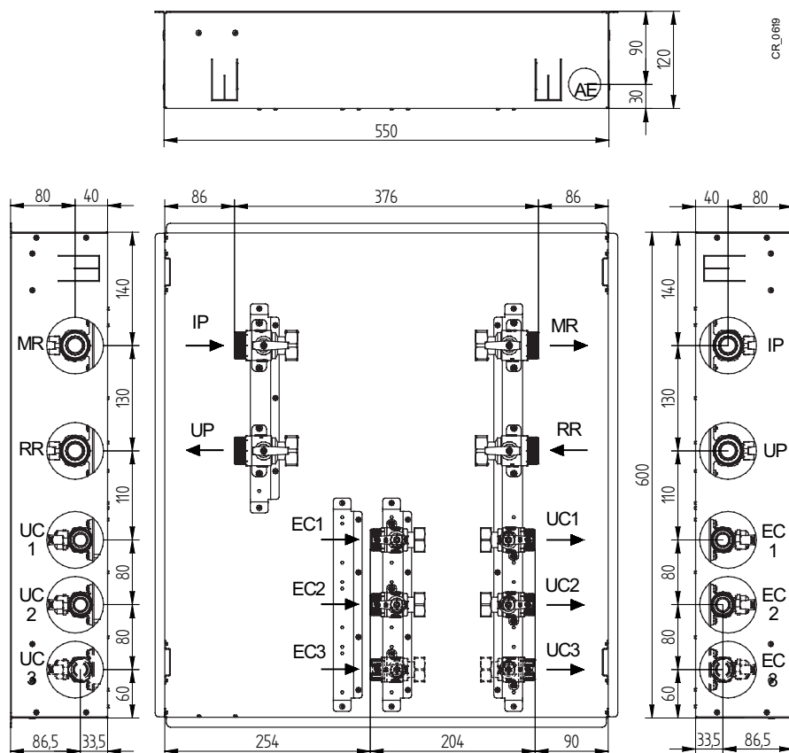
MODEL WITH LITER COUNTER L = 80mm G 3/4"
