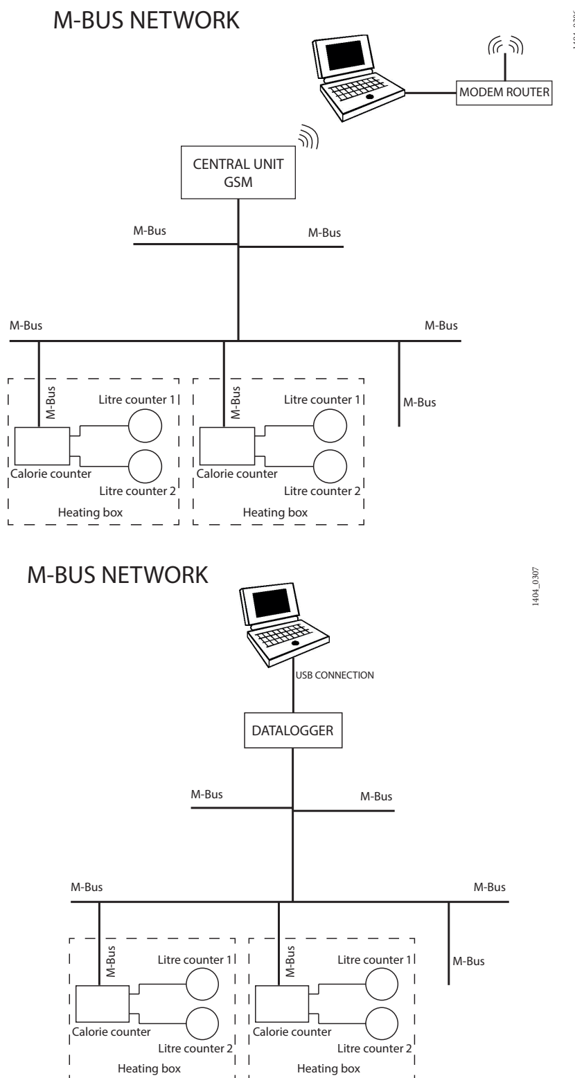
Figura 10B: Diagram of M-Bus network
