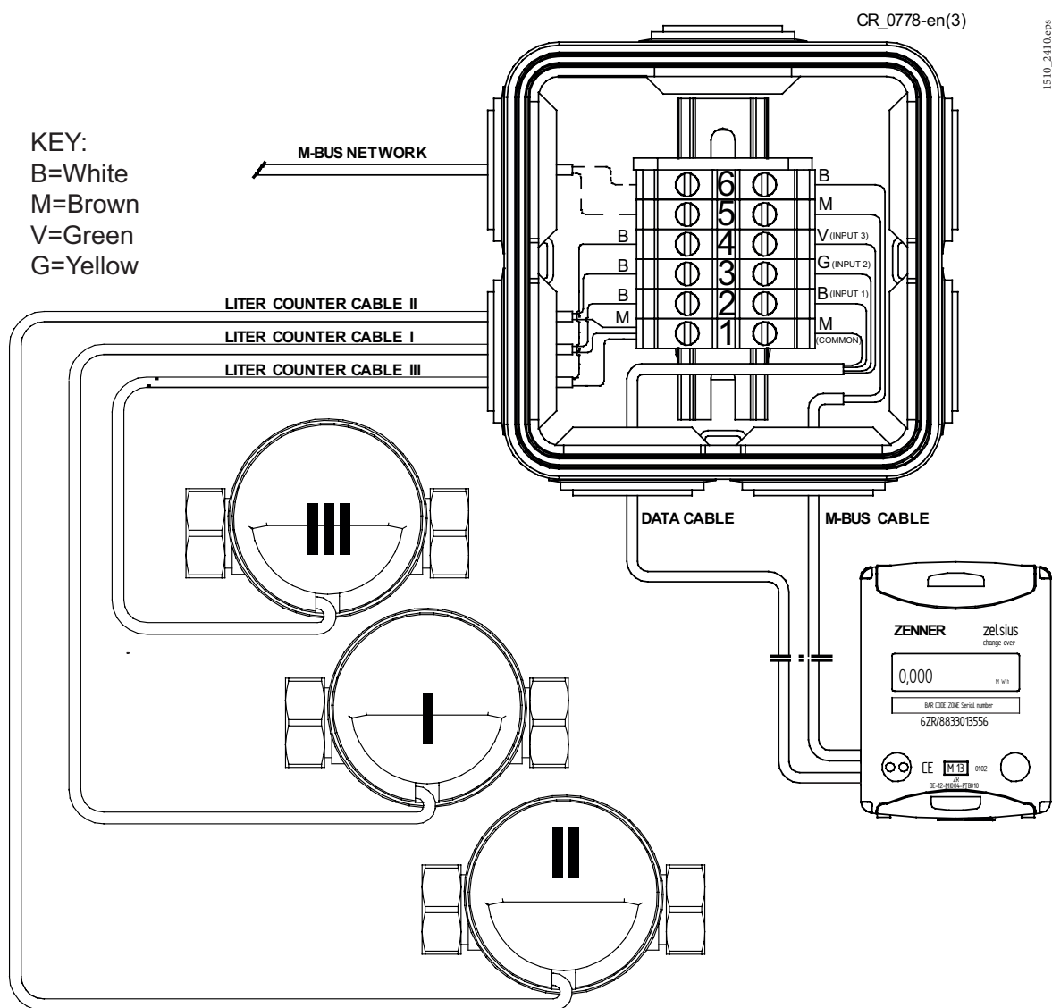
Figure 8B: Connecting liter counter to calorie counter
