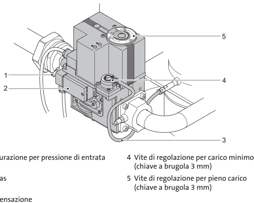
Fig. 28: Valvola gas (Honeywell)
